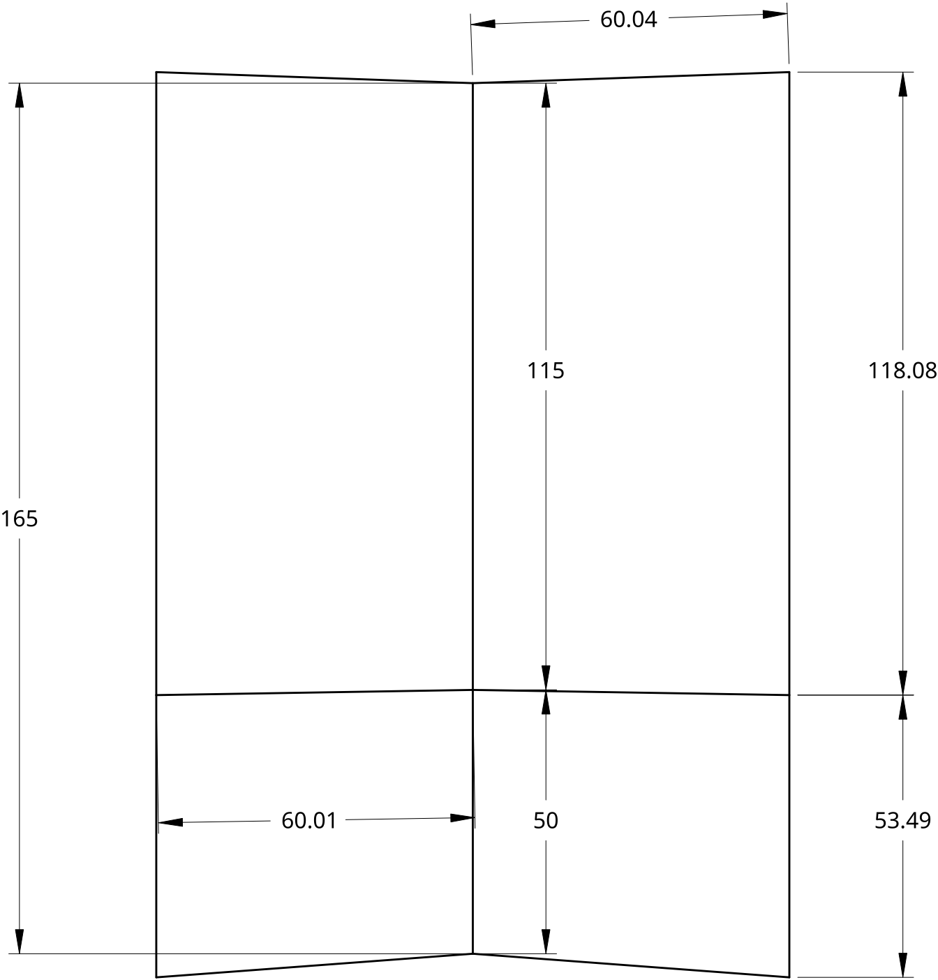
Top View
