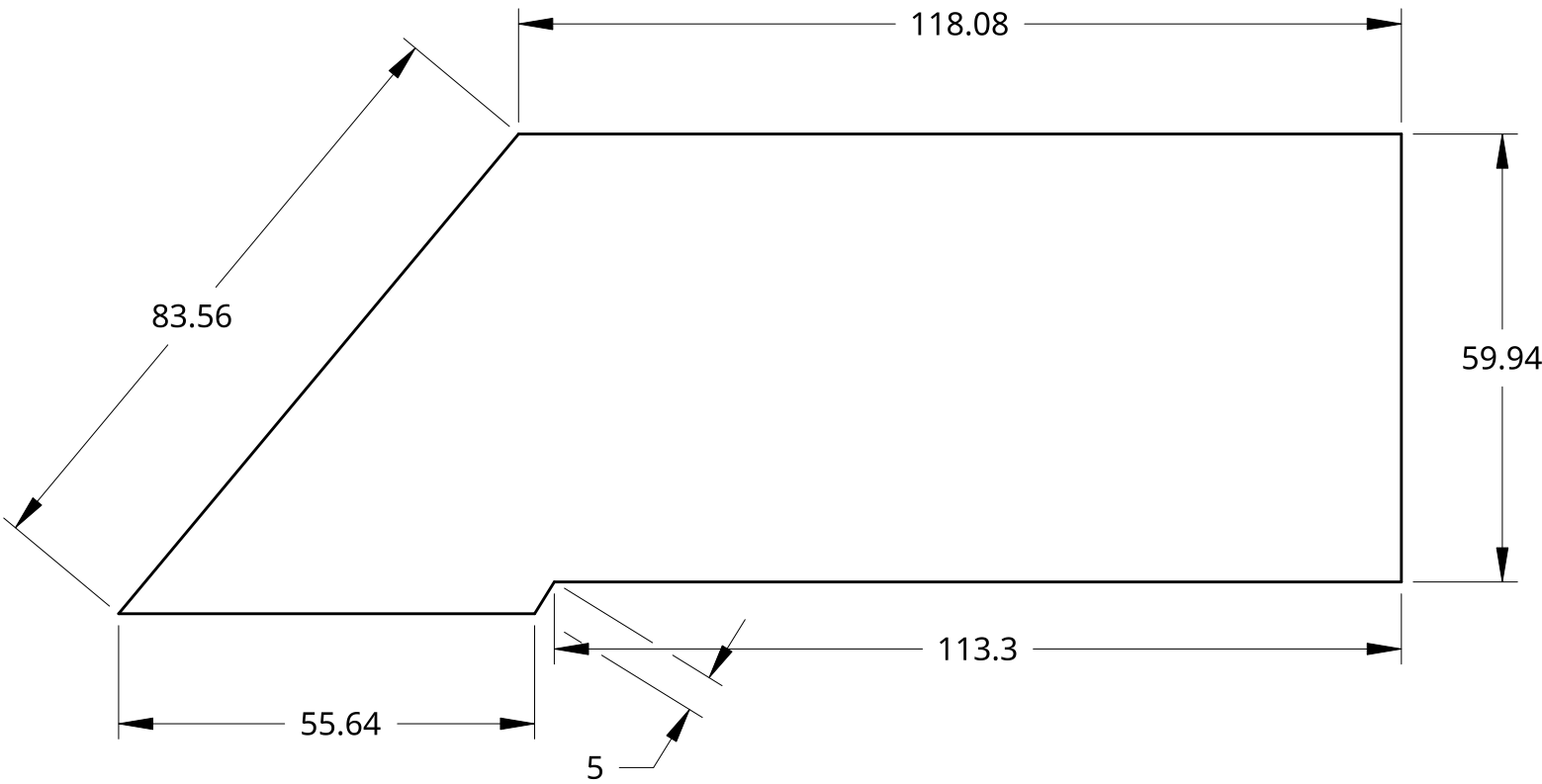
Right View
